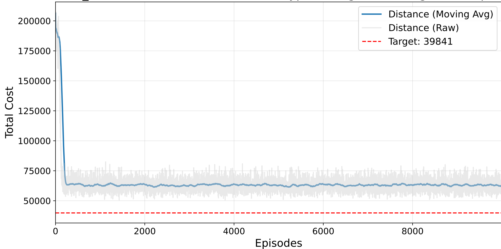
Final NO_BAYESIAN Masked AutoRL-SOP (HyperTuningSK) Training - kro124p.2.sop
